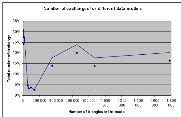
Edges exchanges of the triangular mesh Figure 9
